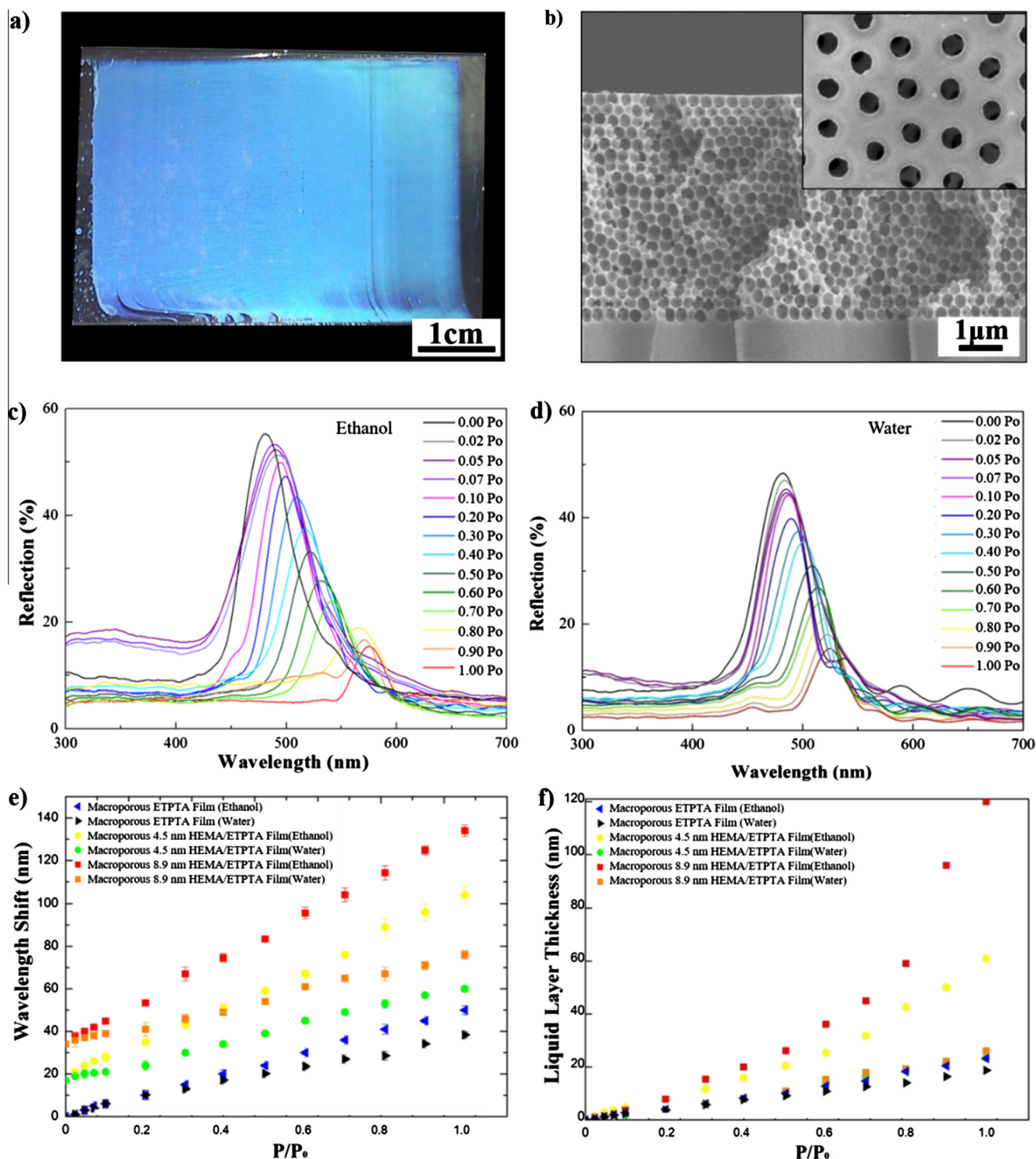
Fig. 4. (a) Photograph of a macroporous thin-PHEMA/PETPTA film templated from 255 nm silica particles. (b) Cross-sectional SEM image of the same sample as in (a). Insert shows a magnified top-view SEM image. (c) Normal-incidence specular reflection spectra obtained from the film exposed to ethanol vapors with different vapor pressures. (d) Normal-incidence specular reflection spectra obtained from the film exposed to water vapors with different vapor pressures. (e) Dependence of the shift of the Bragg diffraction peak on vapor partial pressure. (f) Calculated adsorbed condensed liquid layer thickness at different vapor partial pressures.
