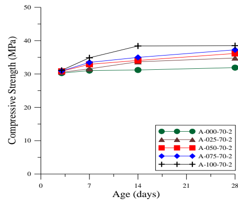
Fig. 5 Compression test on repaired samples with 2-mm crack
