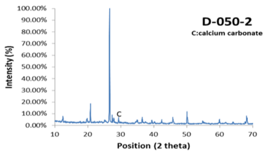
Fig. 7 Day-28 XRD test of the microbe-repaired samples with 50% bacteria and 70% Urea-CaCl 2 medium concentration
