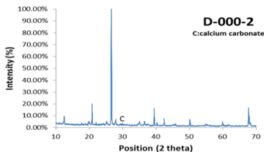
Fig. 8 Day-28 XRD test of the microbe-repaired samples with no bacteria and 70% Urea-CaCl 2 medium concentration
