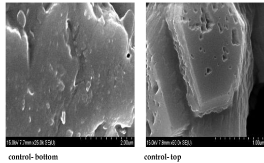
Fig. 10 Day-28 SEM test of the microbe-repaired samples with no bacteria and 70% Urea-CaCl 2 medium concentration
