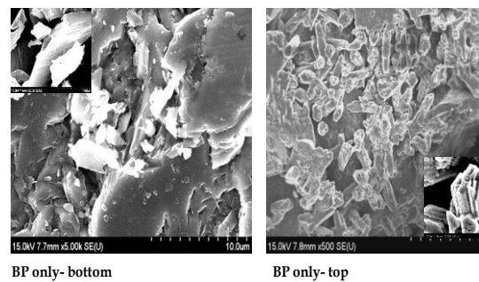
Fig. 11 Day-28 SEM test of the microbe-repaired samples with 100% bacteria and 70% Urea-CaCl 2 medium concentration
