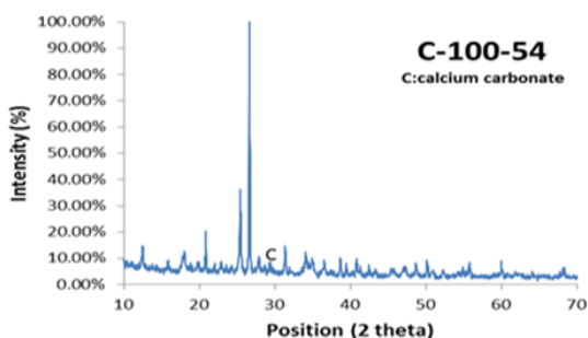
Fig. 9 Day-7 XRD test of the microbe-repaired samples with 100% bacteria and 70% Urea-CaCl 2 medium concentration
