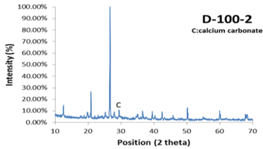
Fig. 6 Day-28 XRD test of the microbe-repaired samples with 100% bacteria and 70% Urea-CaCl 2 medium concentration
